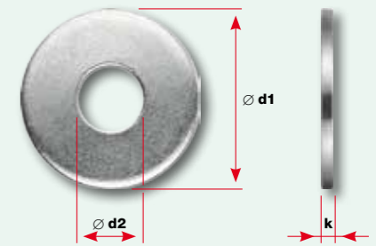
M3-20 (DIN 9021)
